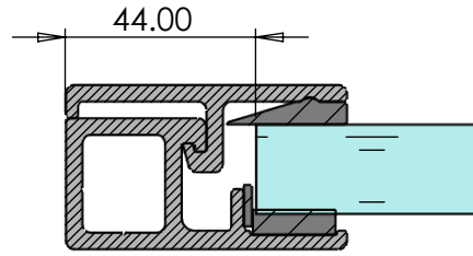
DETAIL B SCALE 1 : 2
